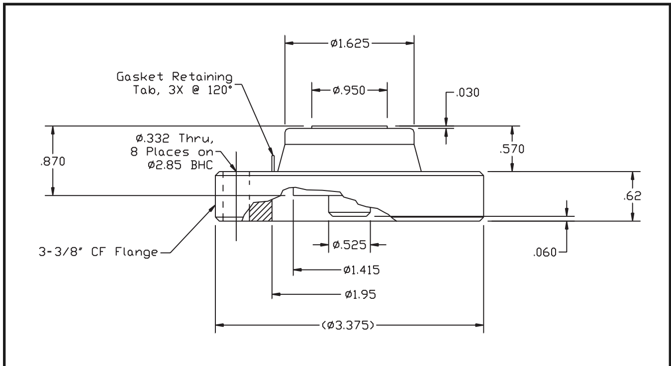
HWEG-101227 Dimensions and Grid Configuration
