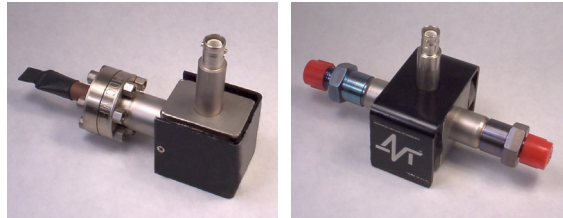
2 L/Sec Ion Pumps with Standard Port Designs
