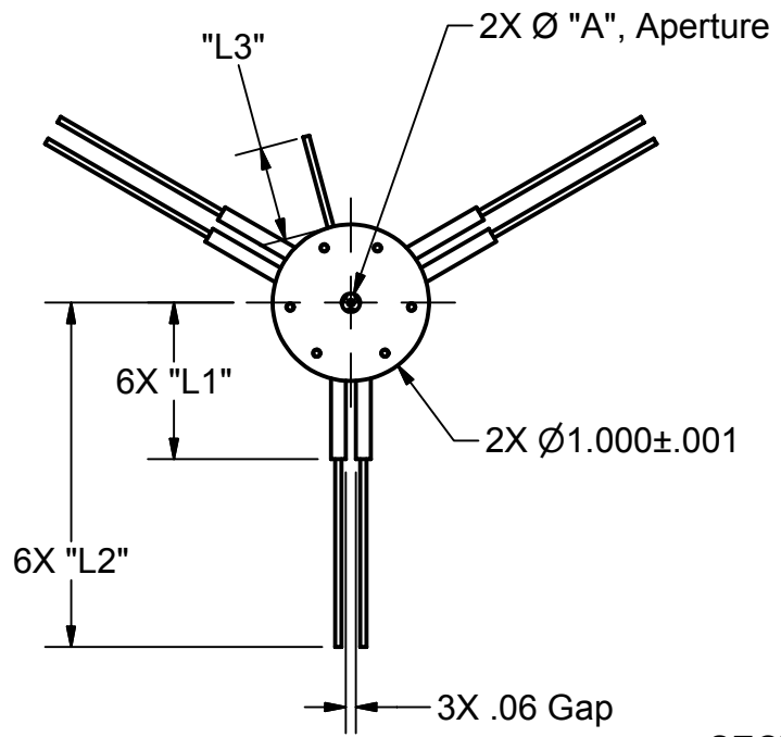
SECTION D-D SCALE 3/4
